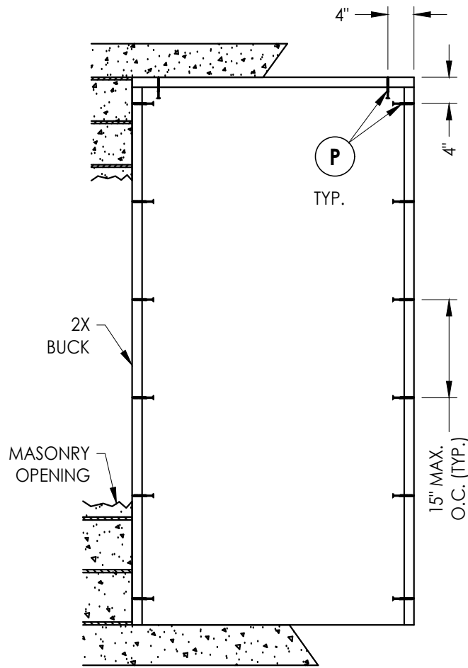
BUCK ANCHORING
